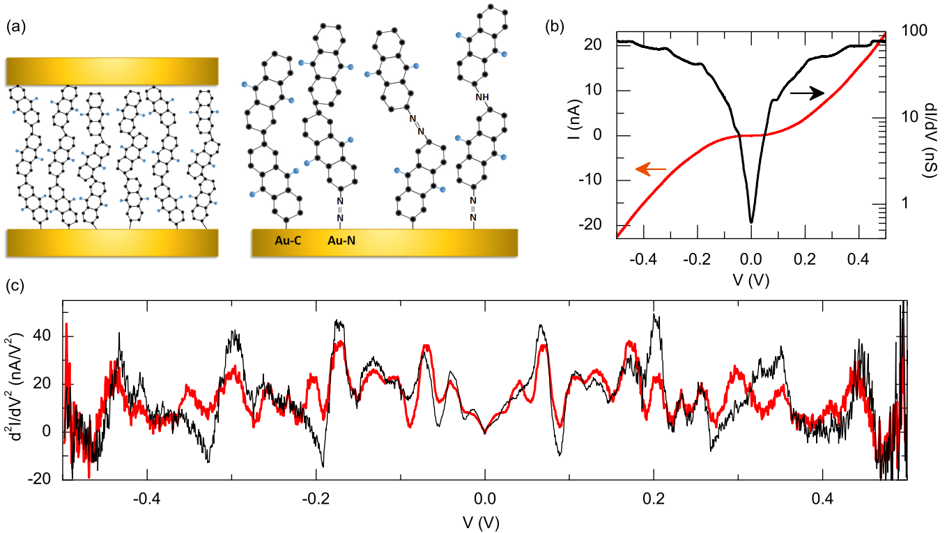
FIG. 1. (a) Simplified picture of the AQ based molecular junction and scheme of the possible covalent bonds (Au-C and Au-N) between the molecular layer and the base electrode induced by electrografting together with azo-based molecule-molecule bonds in the layer revealed by transport measurements. (b) Current-voltage characteristics I(V) (red) and differential conductance G(V) (black) as a function of voltage in an AQ based junction measured at 5 K. The junction area is \sim 20 \times 100 \mu\text{m}^2 and the molecular layer thickness is \sim 8 nm. (c) Measurement of the second derivative of the current d^2I/dV^2 as function of the voltage V for the same junction at 5 K (black curve). The same data after symmetrization is superposed (red curve).
